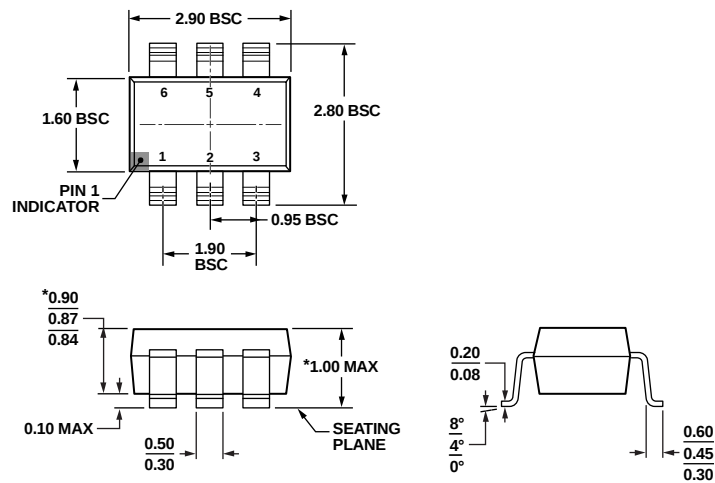
*COMPLIANT TO JEDEC STANDARDS MO-193-AA WITH THE EXCEPTION OF PACKAGE HEIGHT AND THICKNESS. Figure 31.. 6-Lead Thin Small Outline Transistor Package [TSOT] (UJ-6) Dimensions shown in millimeters
