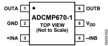
Figure 3. Pin Configuration
