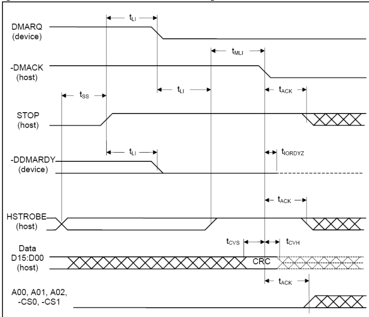
Figure 18: Ultra DMA Data-Out Burst Device Termination Timing
