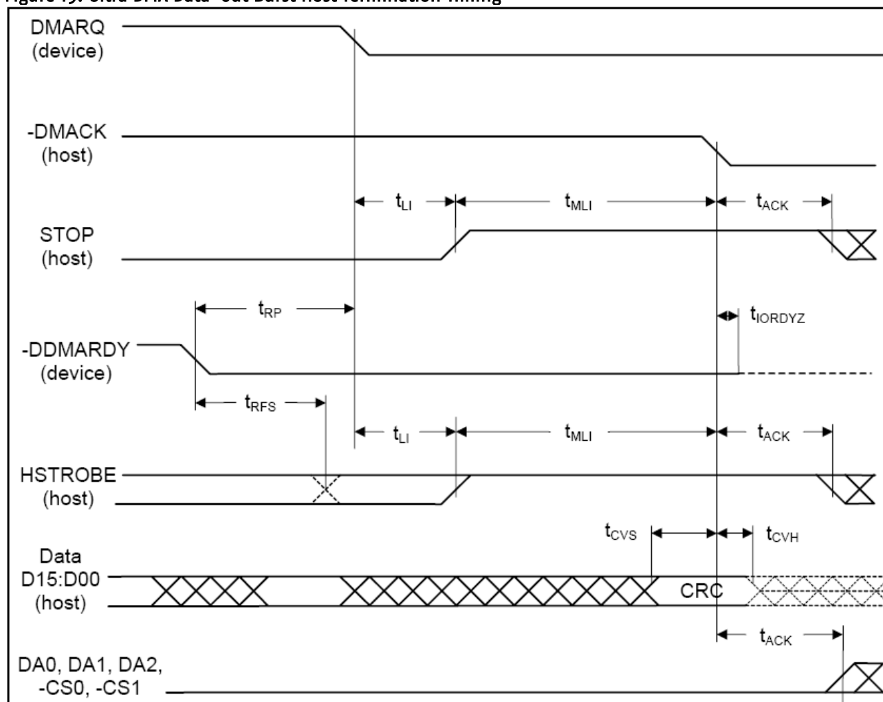
Figure 19: Ultra DMA Data-Out Burst Host Termination Timing
