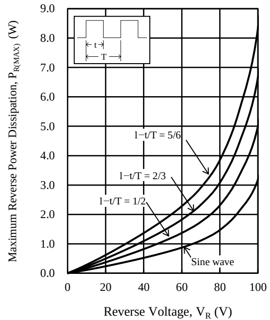
Figure 4. P_{R(MAX)} vs. V_R ( T_J = 150\text{ °C} )
