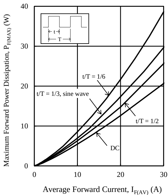
Figure 3. P_{F(MAX)} vs. I_{F(AV)} ( T_J = 150\text{ °C} )
