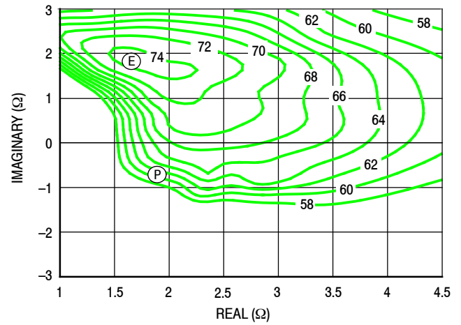
Figure 25. P1dB Load Pull Efficiency Contours (%)
