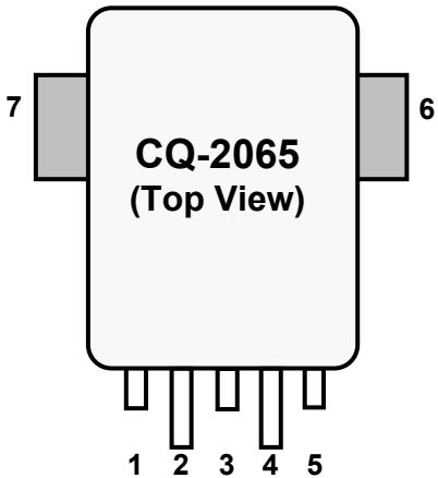
Figure 3. Pin-out diagram
