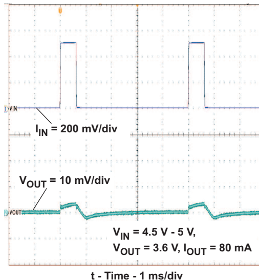
Figure 18. Line Transient
