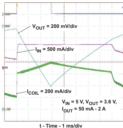
Figure 17. Load Transient
