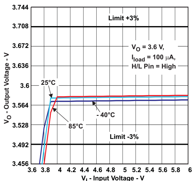
Figure 12. Output Voltage vs Input Voltage
