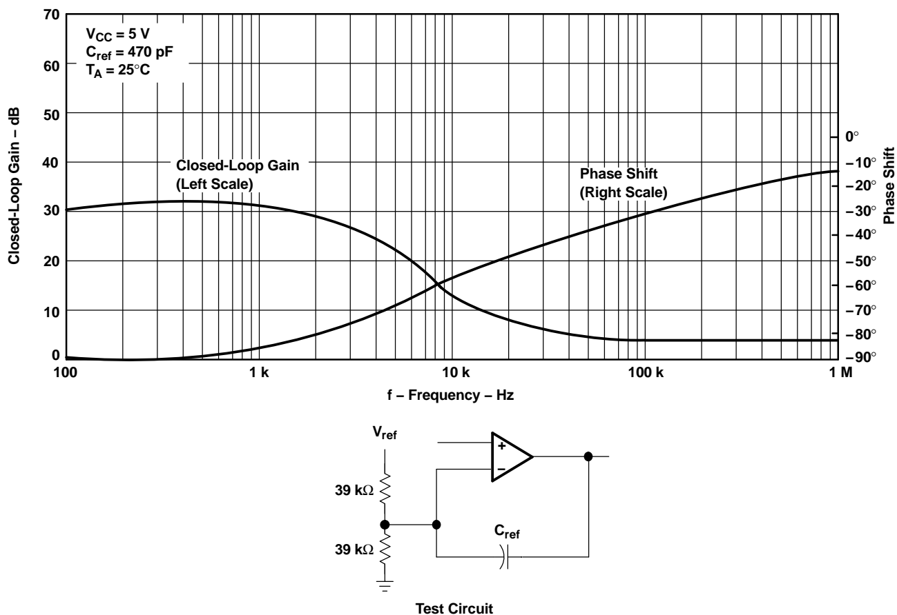
Figure 22. Closed-Loop Gain and Phase Shift vs Frequency
