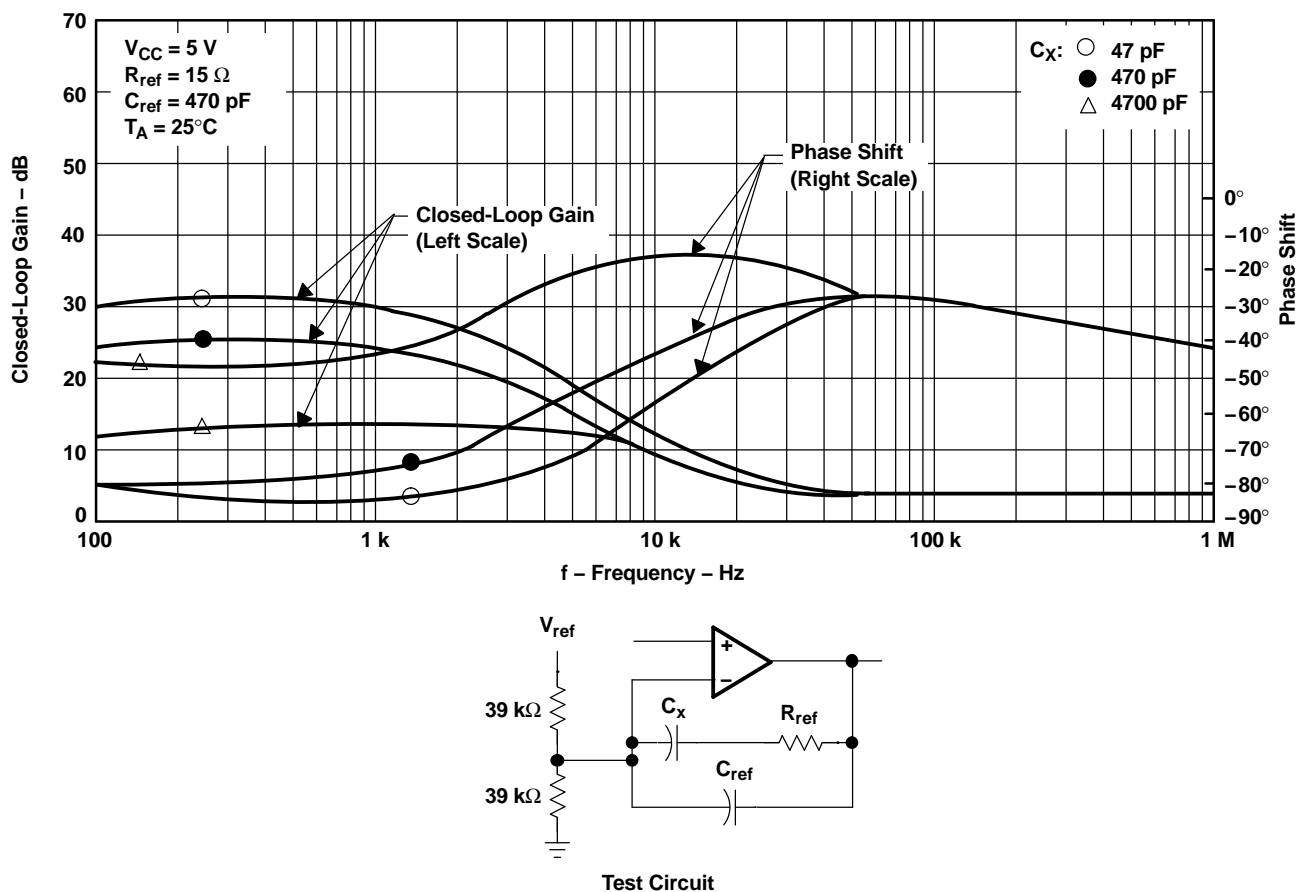
Figure 20. Closed-Loop Gain and Phase Shift vs Frequency
