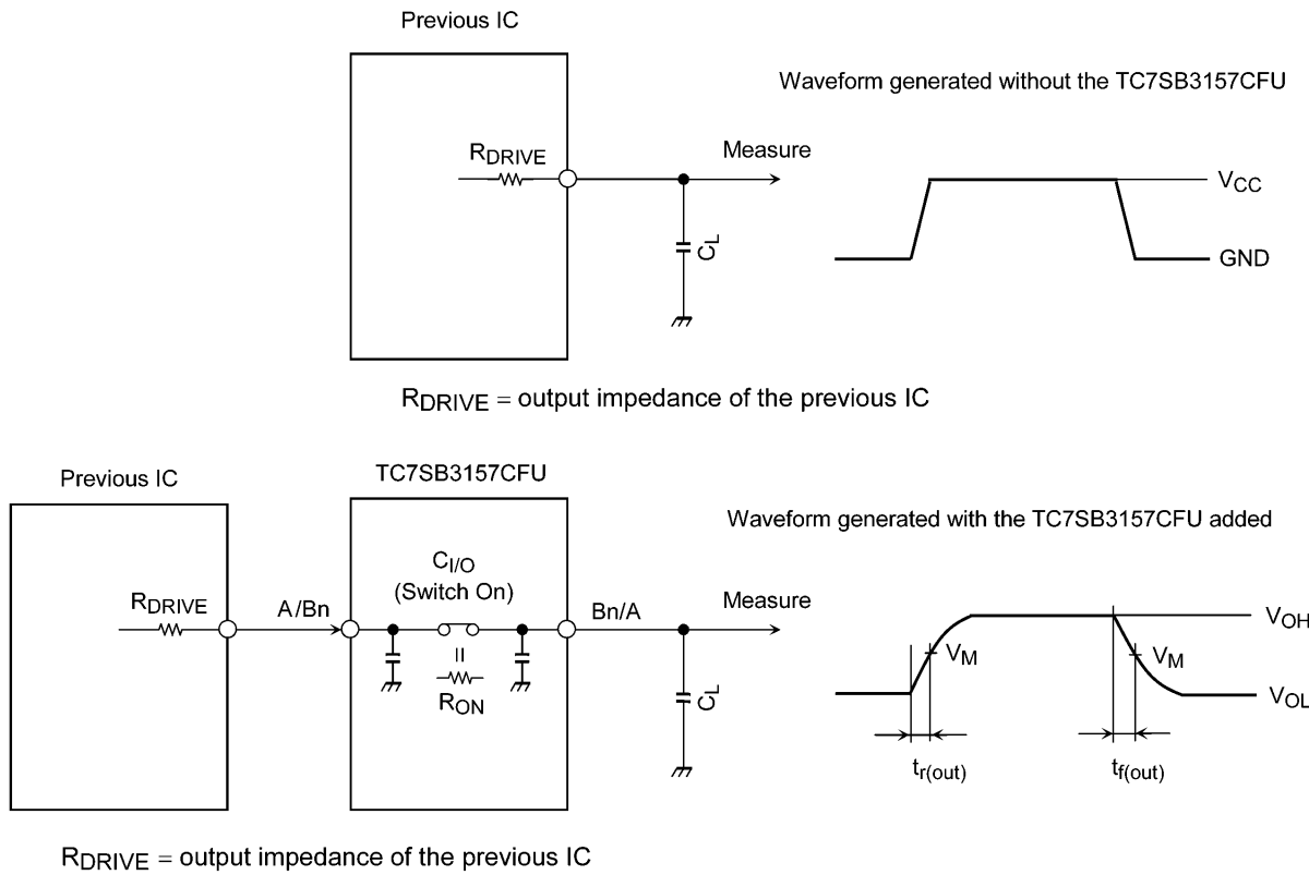
Fig. 11.1 Calculation Circuit
