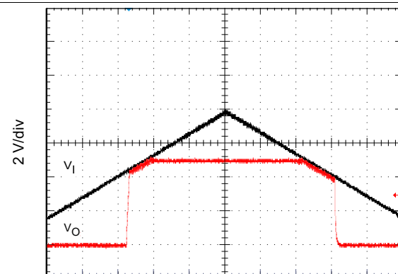
Figure 58. Low-Dropout Operation
