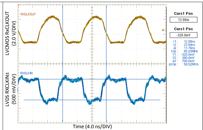
Figure 25. LVDS CLKIN Aligned With LVCMS RxCLKOUT
