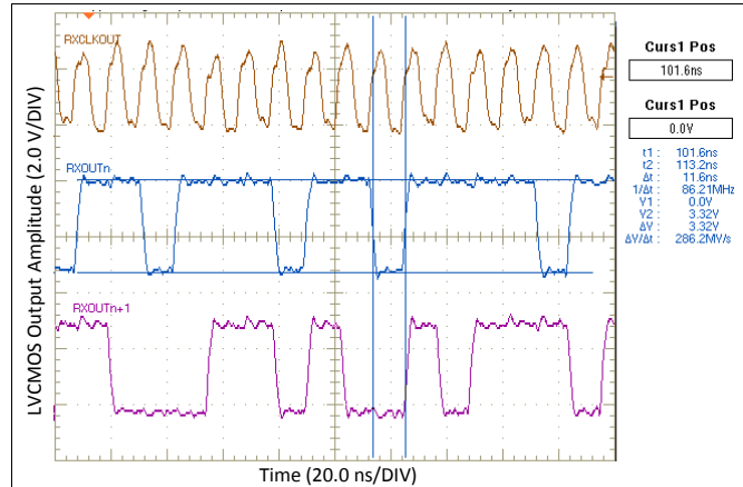
Figure 14. Parallel PRBS-7 on LVCMOS Outputs at 85 MHz
