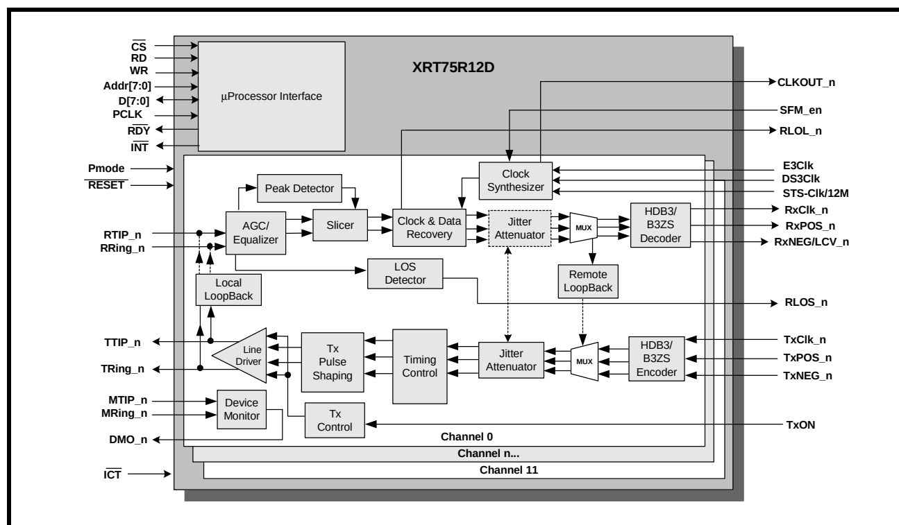
FIGURE 1. BLOCK DIAGRAM OF THE XRT 75R12D
