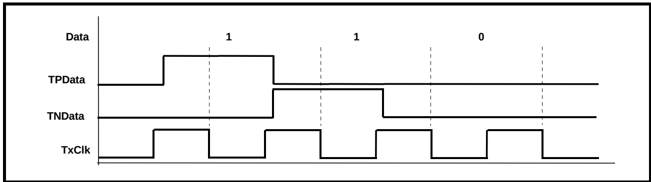
FIGURE 26. DUAL-RAIL DATA FORMAT (ENCODER AND DECODER ARE DISABLED)
