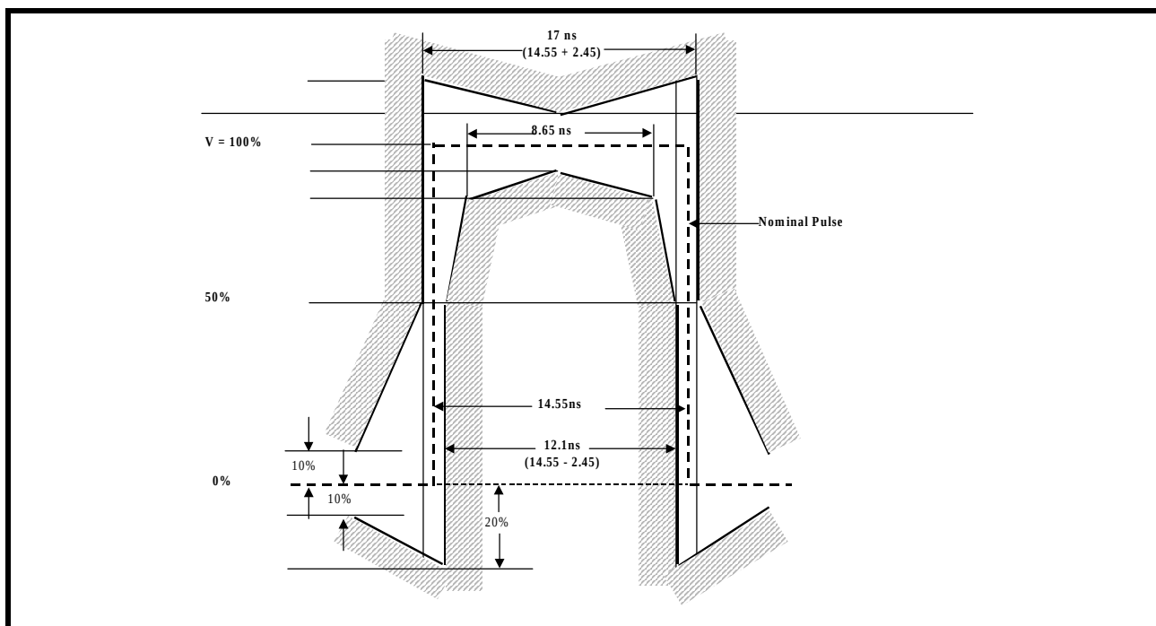
FIGURE 30. PULSE MASK FOR E3 (34.368 MBITS/S) INTERFACE AS PER ITU-T G.703
