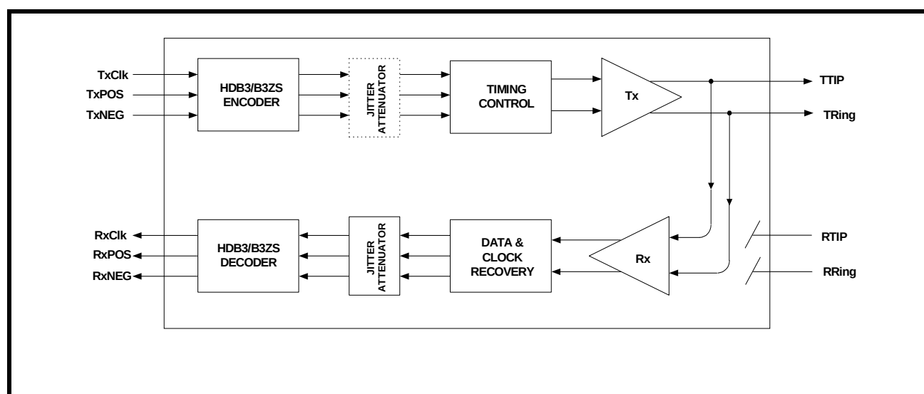
FIGURE 18. ANALOG LOOPBACK
