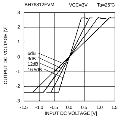
Fig. 33 Output DC voltage – Input DC voltage
