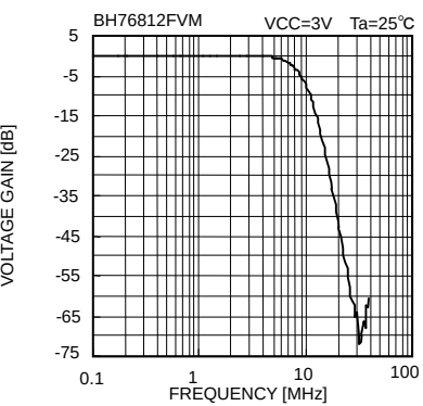
Fig. 22 Frequency characteristic
