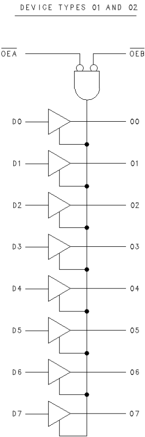
FIGURE 3. Logic diagram.
