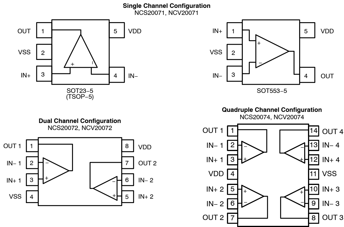
Figure 1. Pin Connections
