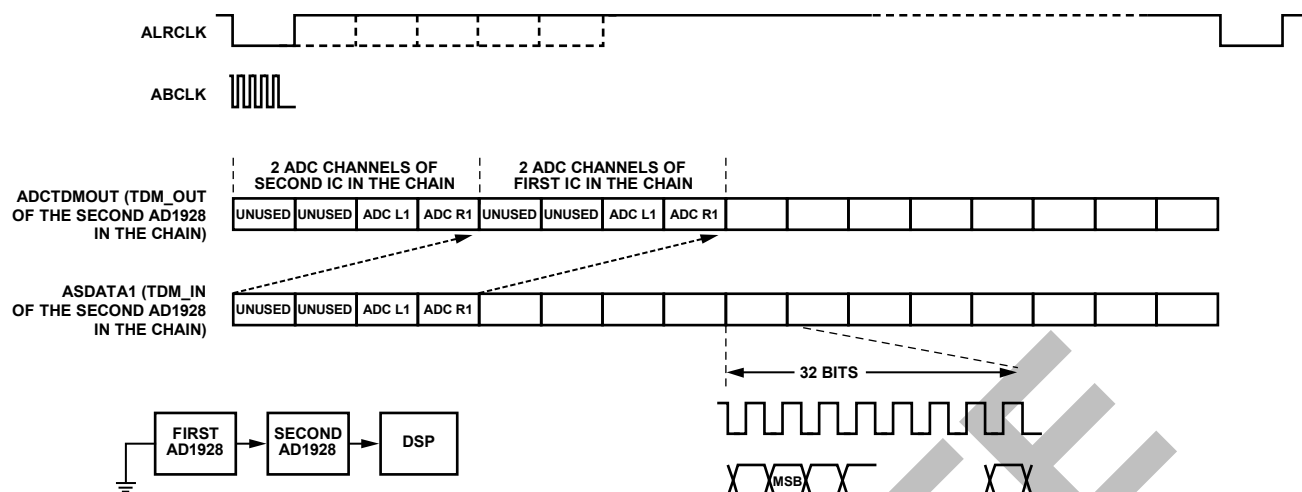
Figure 22. ADC TDM Daisy-Chain Mode (512 f_s BCLK, Two-AD1928 Daisy Chain)
