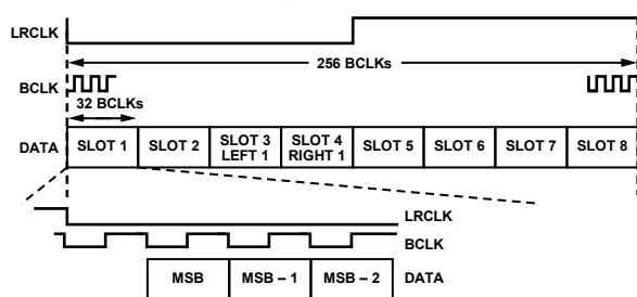
Figure 12. ADC TDM (6-Channel I 2 S Mode)
