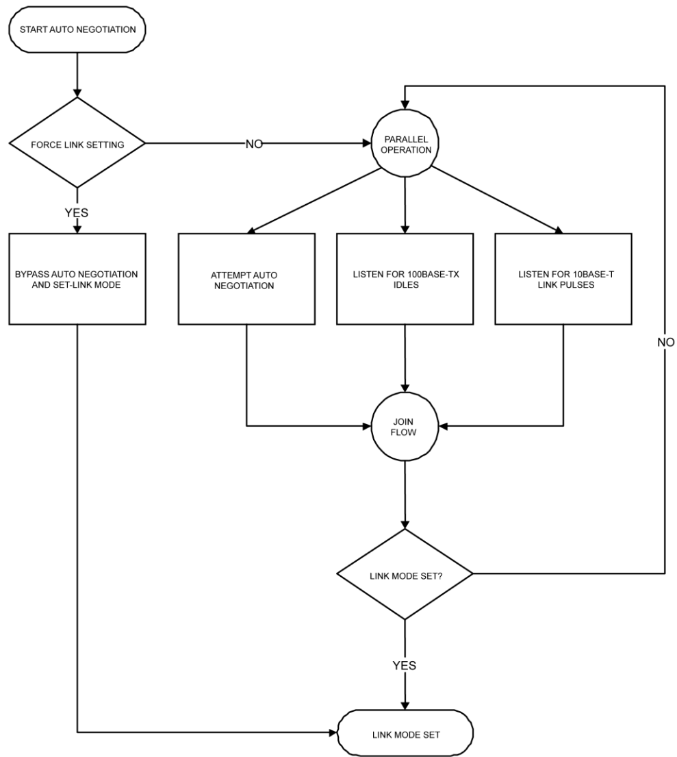
Figure 3. Auto-Negotiation
