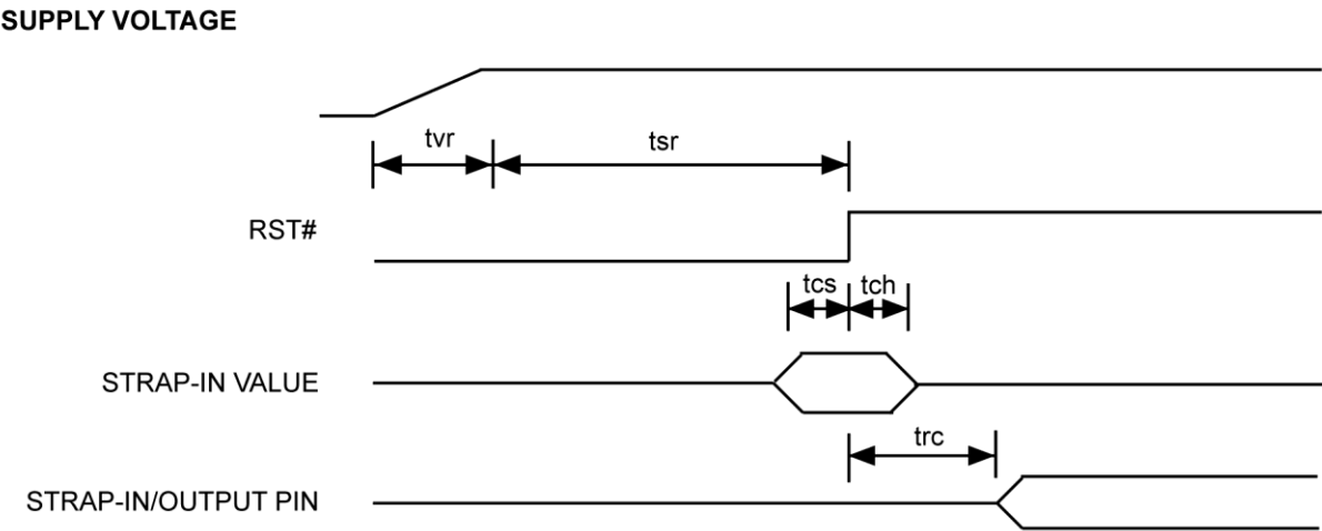
Figure 24. Reset Timing
