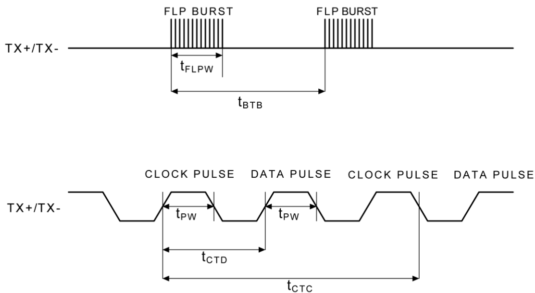
Figure 23. Auto-Negotiation Timing
