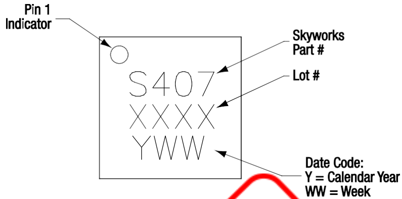
Figure 10. Typical Part Markings (Top View)
