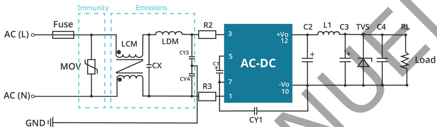
Circuit 5
