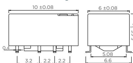
SMT Short Gull wings version
