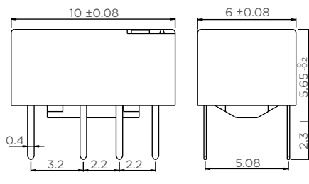
THT Short version
