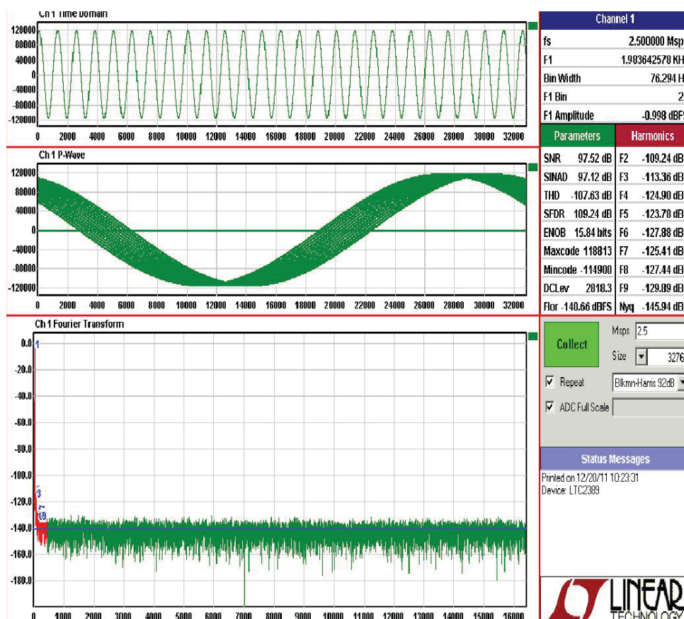
Figure 7. PSCOPE Screenshot
