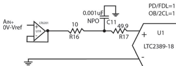
Figure 2. Default Driver Circuit
