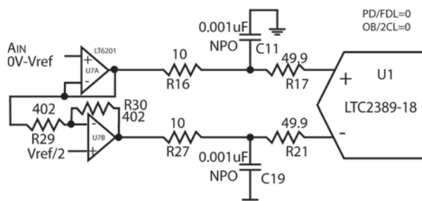
Figure 2. Default Driver Circuit
