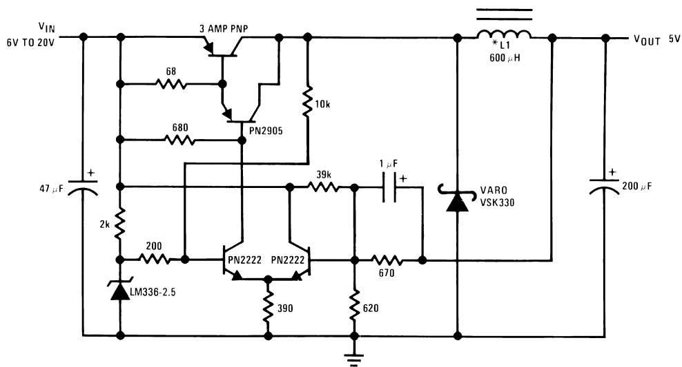
Low Cost 2 Amp Switching Regulator†
