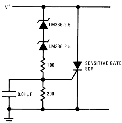
5V Crowbar
