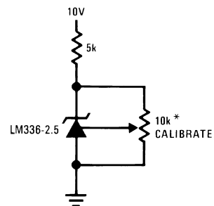
Trimmed 2.5V Reference with Temperature Coefficient Independent of Breakdown Voltage
