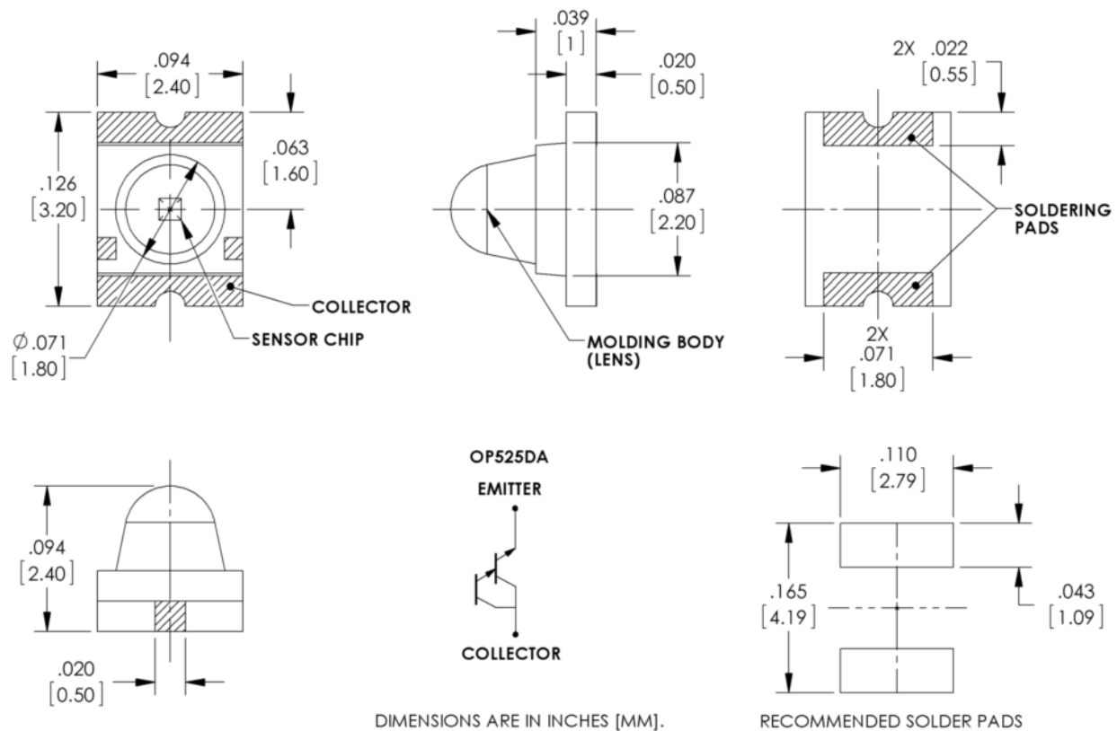
RECOMMENDED SOLDER PADS
