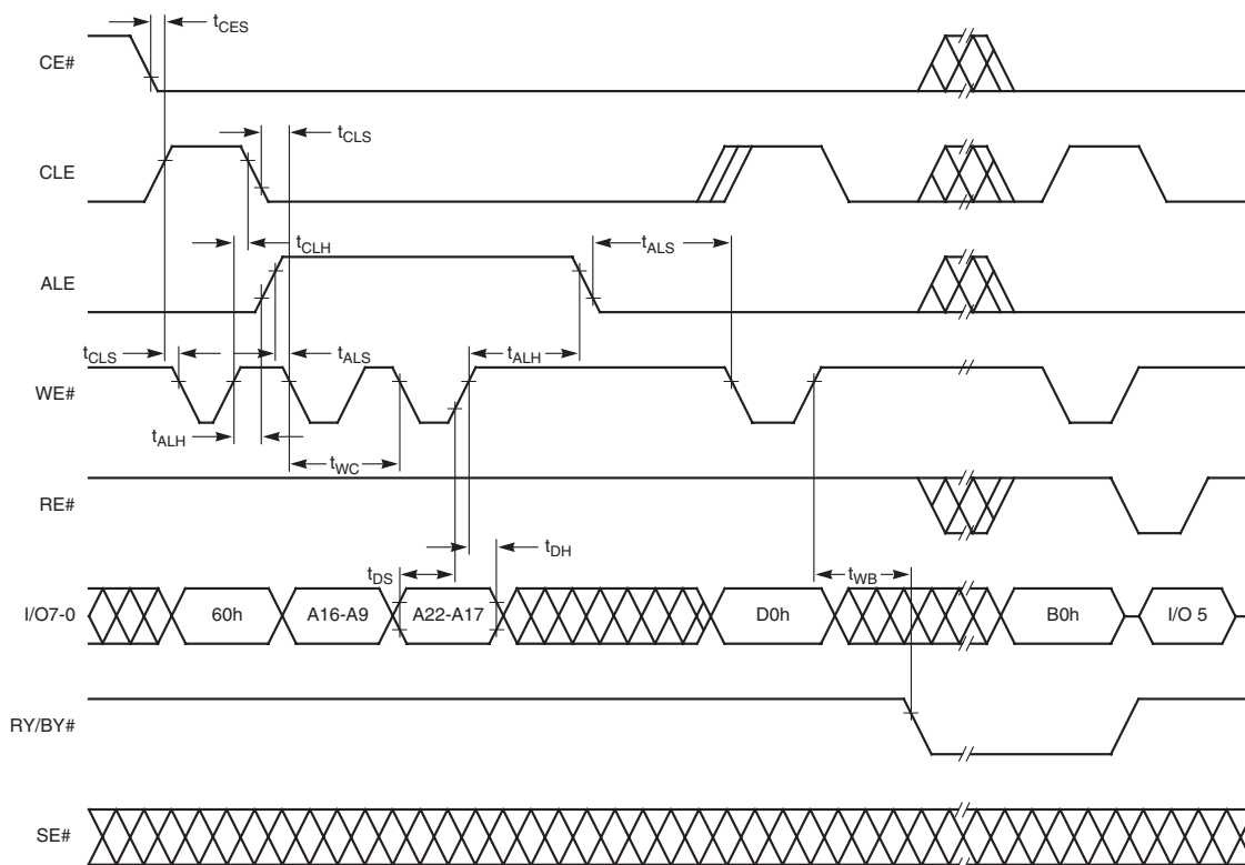
Figure 27. Erase Suspend
