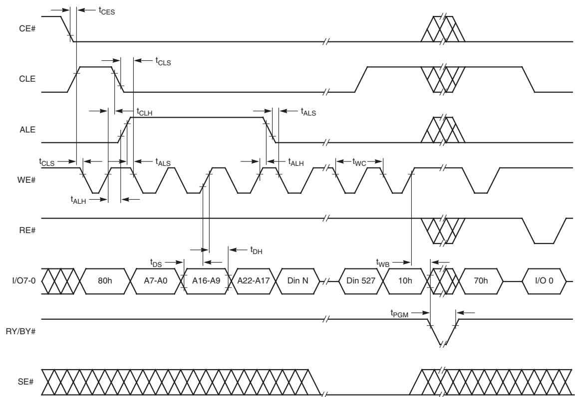
Figure 25. Page Program
