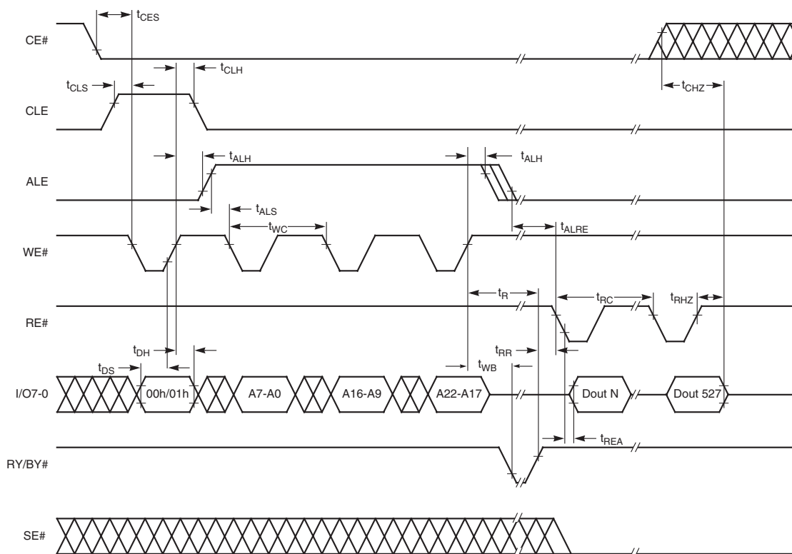
Figure 22. Read Data (Interrupted by \text{CE}\# )
