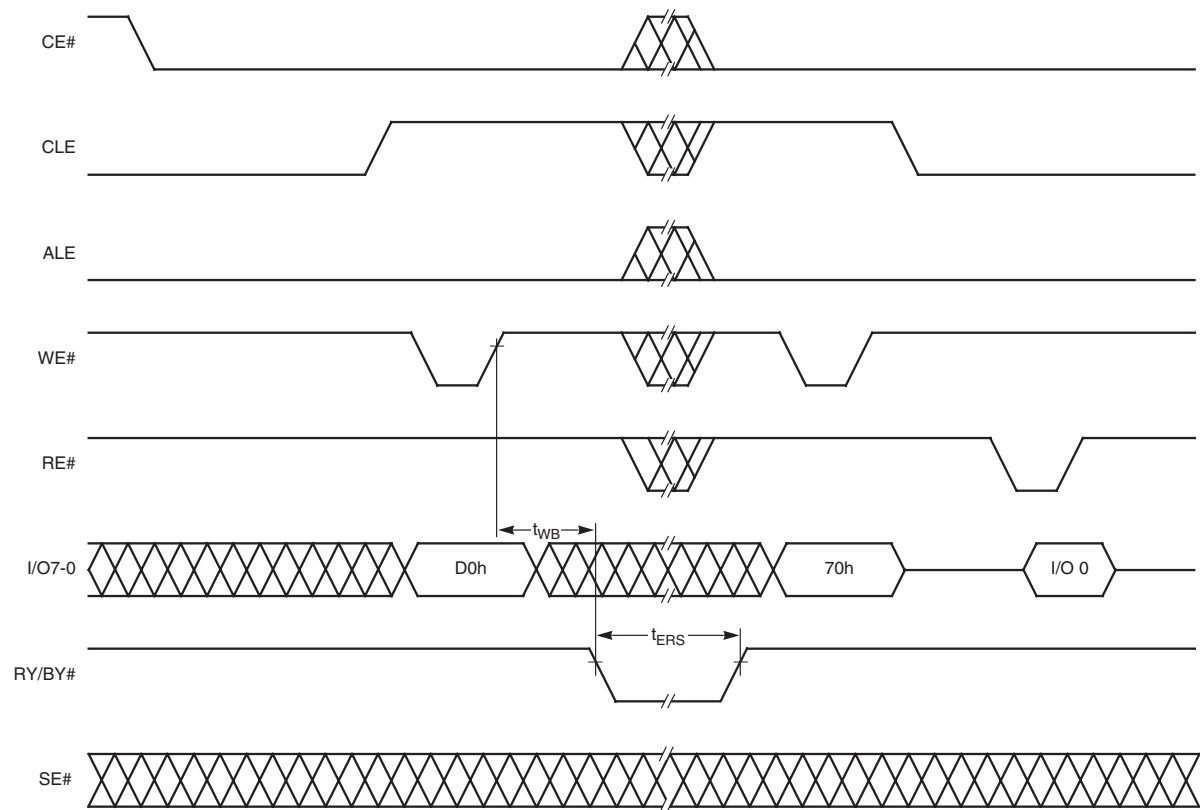
Figure 28. Erase Resume
