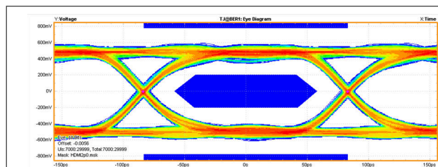
Figure 8-8. 6-Gbps HDMI 2.0 (TP1) Eye Diagram TPD4E05U06
