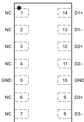
Figure 5-4. RVZ Package 14-Pin USON Top View
