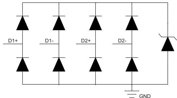
TPD4E05U06 Functional Block Diagram
