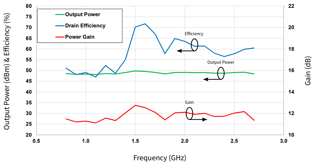
Figure 4. Power, Drain Efficiency and Gain vs Frequency of CGHV27060MP-AMP3 P_{IN} = 37 dBm, V_{DD} = 50 V, I_{DQ} = 120 mA
