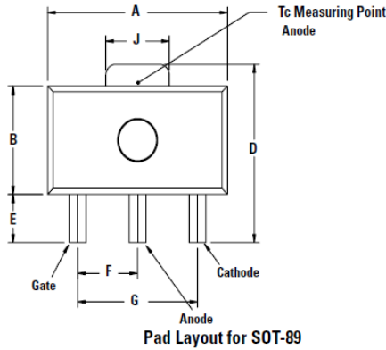
Pad Layout for SOT-89
