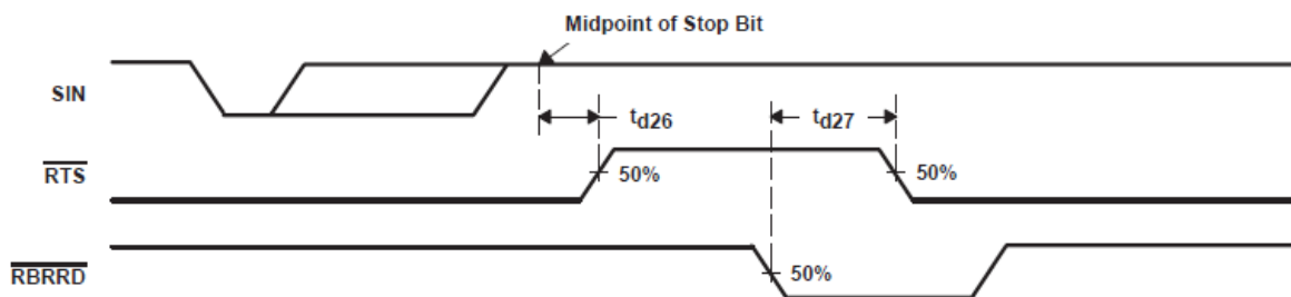
Figure 6-14. Auto-RTS Timing for RCV Threshold of 1, 4, or 8 Waveforms
