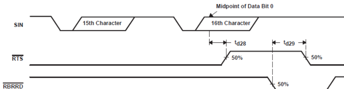
Figure 6-15. Auto-RTS Timing for RCV Threshold of 14 Waveforms
