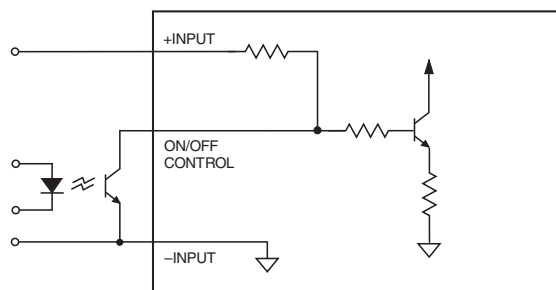
Figure 3. Driving the Negative Polarity On/Off Control Pin
