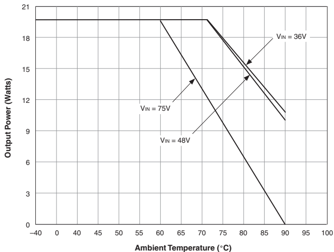
Temperature Derating Curves for UEP-3.3/6000-D48
