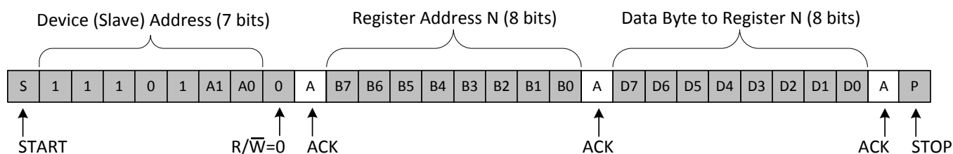
Figure 29. Write to Register
