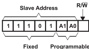
Figure 27. TCA9539 Address
