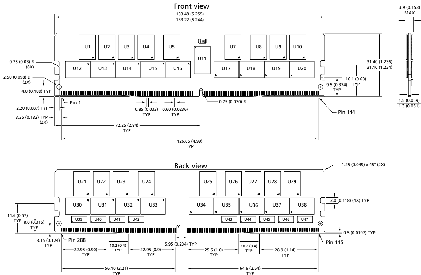
Figure 4: 288-Pin DDR4 LRDIMM
