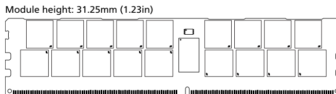
Figure 2: 288-Pin LRDIMM (R/C-E2)
