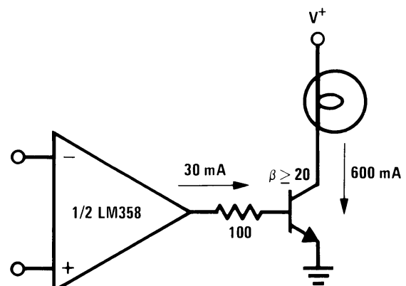
Figure 8-6. Lamp Driver
