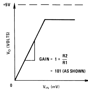
Figure 8-2. Transfer Curve for Non-Inverting Configuration
