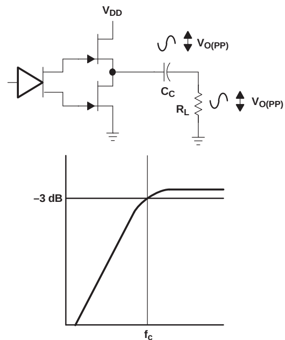
Figure 32. Single-Ended Output and Frequency Response
