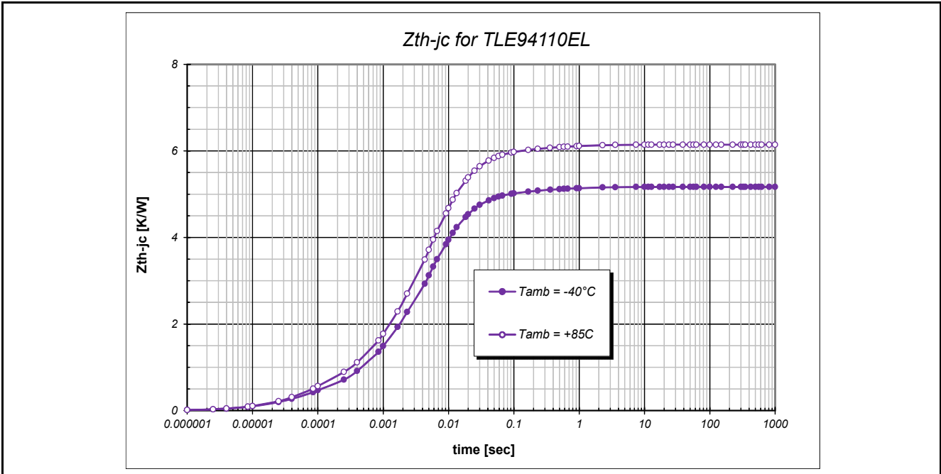
Figure 30 ZthJC Curve
