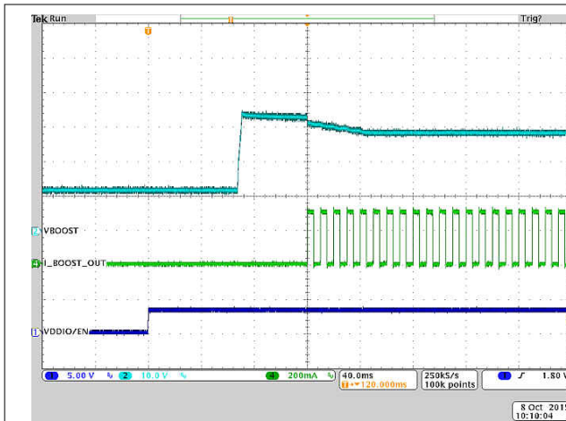
Figure 8-4. Typical Start-Up
