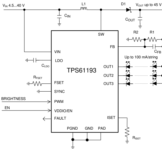
Simplified Schematic
