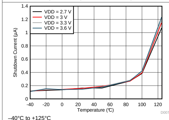
Figure 6. Shutdown Mode I_{DD} vs Temperature
