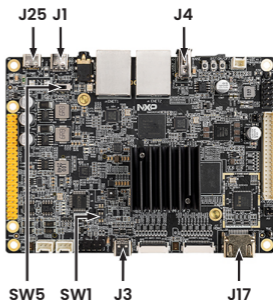
Figure 3: Available connections and switches to get started with the FRDM i.MX 95 development board
