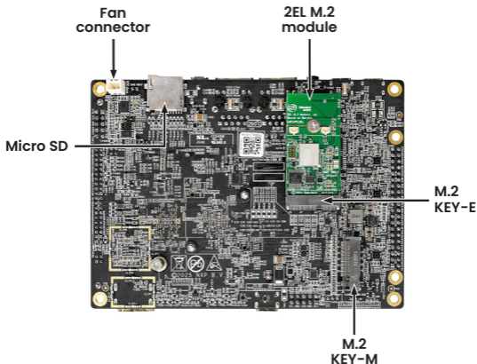
Figure 2: Bottom view of the FRDM i.MX 95 development board
