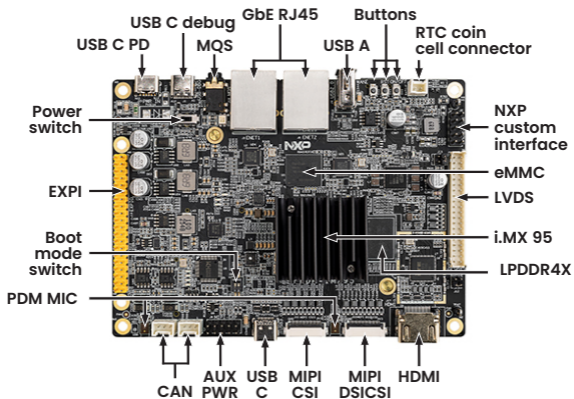
Figure 1: Top view of the FRDM i.MX 95 development board
