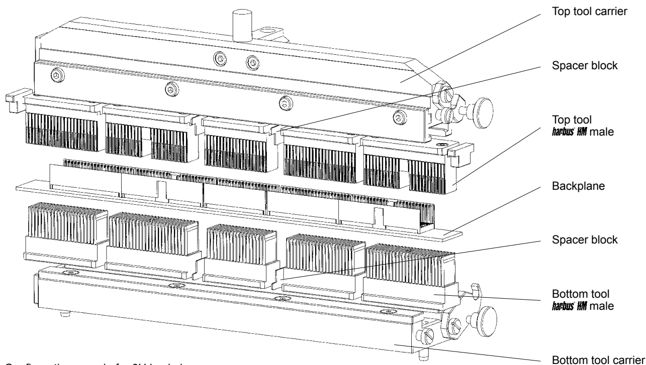
Configuration sample for 6U backplane
