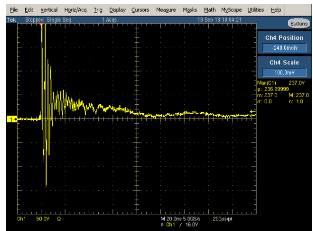
Figure 15. Positive 12 kV IEC
