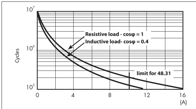
F 48 - Electrical life (AC) v contact current
