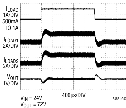
Load Step
