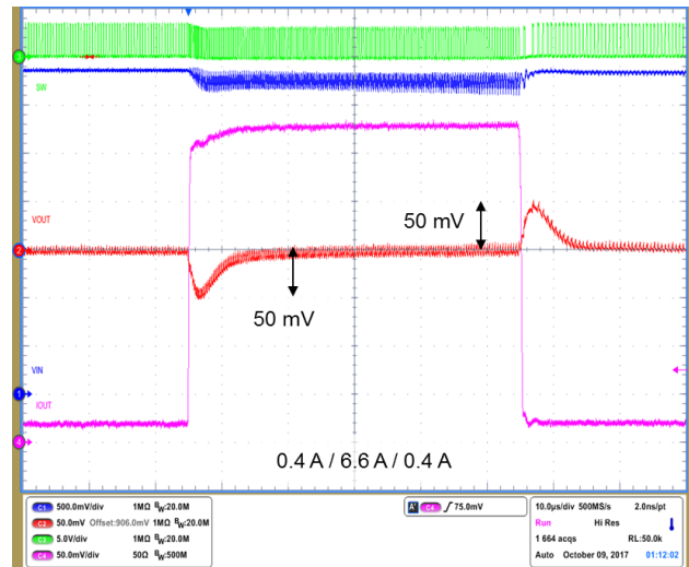
Figure 35. Transient Load 0.4 to 6.6 A – Forced PWM, V_{IN} = 3.3\text{ V} – V_{OUT} = 1.0\text{ V} – L = 0.24\text{ uH} – C_{OUT} = 4 \times 47\text{ uF}
