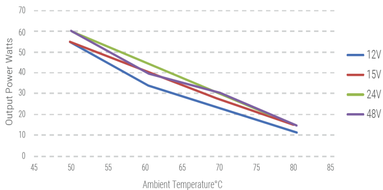
MB60 Series Output Power Derating
