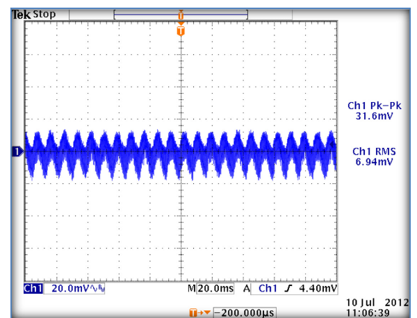
24V Out, Full load, 264VAC, 50Hz
