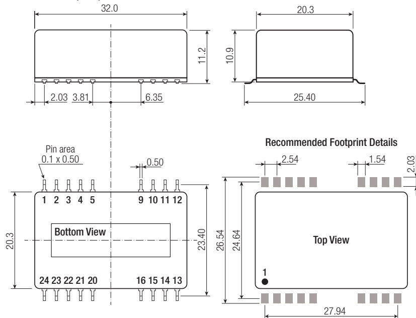
Dimension Drawing SMD metal case (mm)
