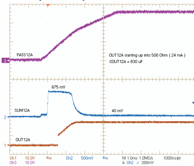
Figure 17. OUT12A Startup Into 500-Ω, 830-µF Load
