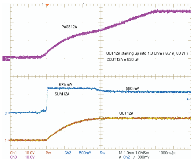
Figure 18. OUT12A Startup Into 80-Watt, 830-µF Load
