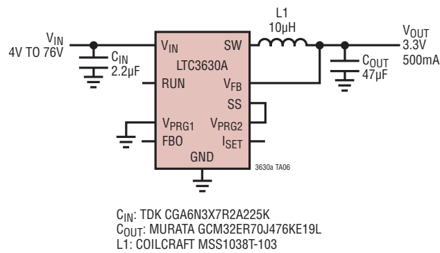
4V to 76V Input to 3.3V Output, 500mA Step-Down Converter
