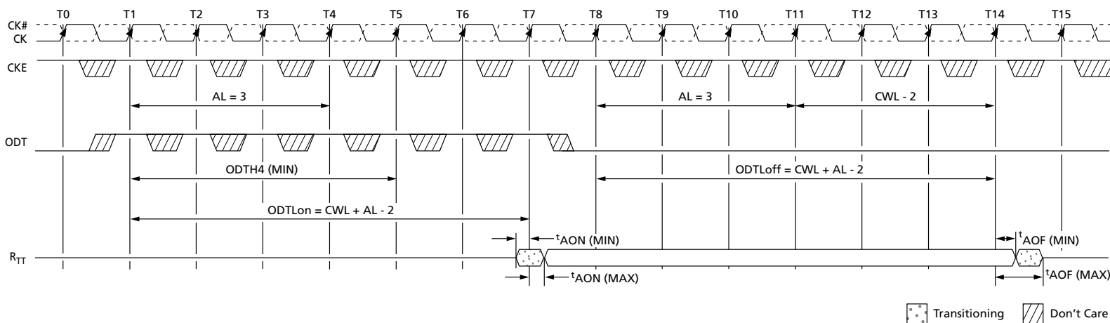
Figure 112: Synchronous ODT
