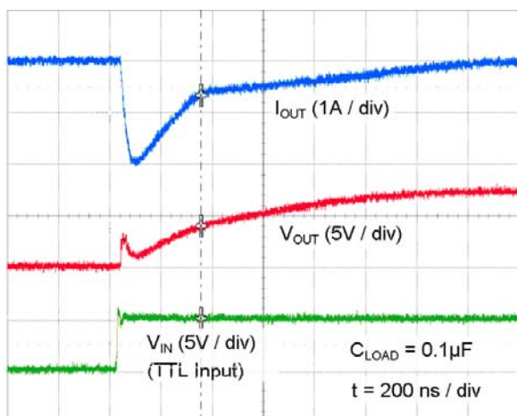
Figure 45. Quasi-Static Source Current with V_{DD}=12 V
