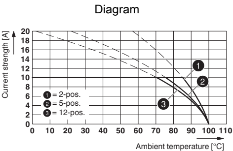
Type: FKCS 2,5/...-ST with MDSTBW 2,5/...-G
