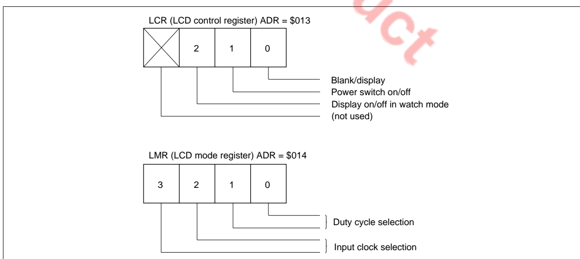
Figure 36 LCD Control Register
