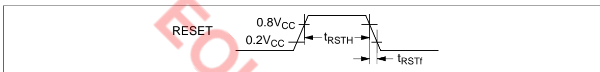
Figure 45 Reset Timing
