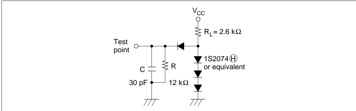
Figure 47 Timing Load Circuit
