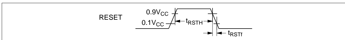
Figure 50 Reset Timing
