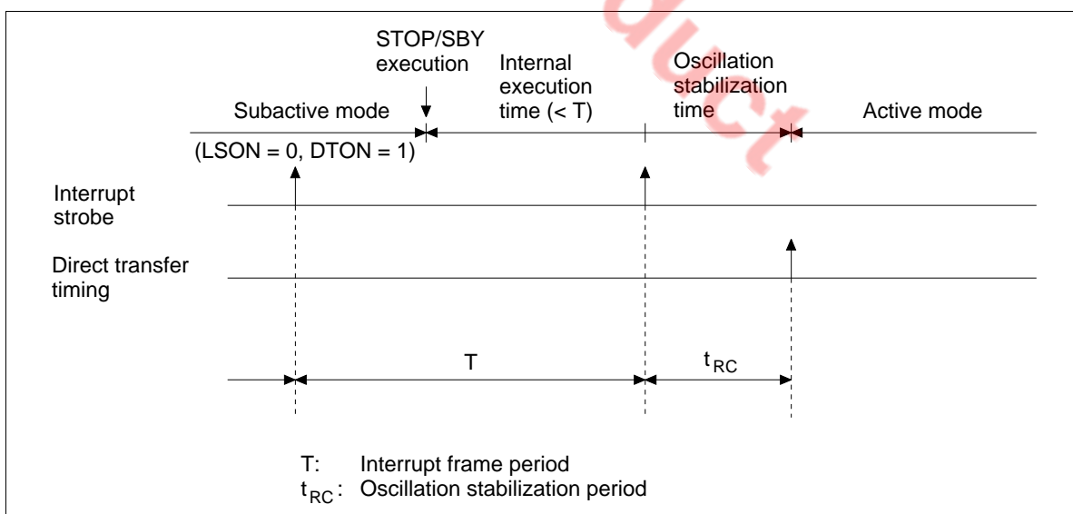
Figure 14 Direct Transfer Timing
