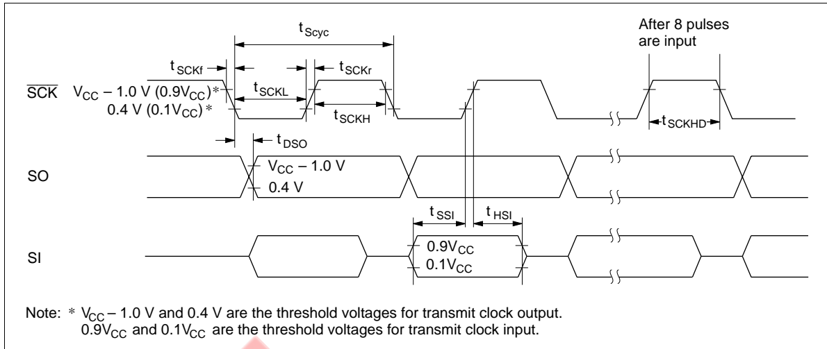
Figure 51 Timing of Serial Interface
