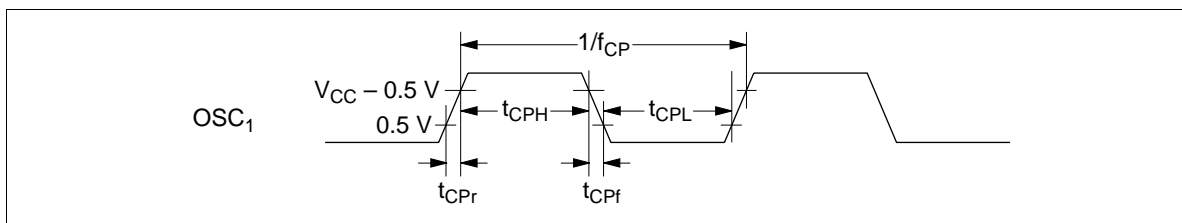
Figure 43 Oscillator Timing
