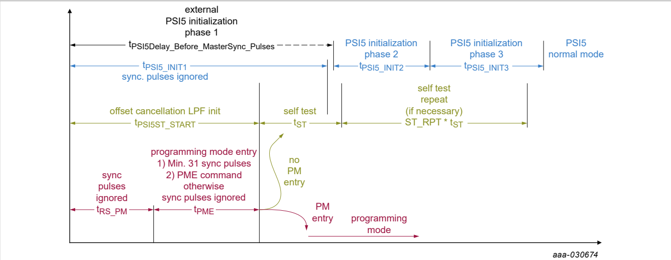
Figure 89. PSI5 initialization timing, synchronous mode
